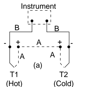
Schematic Wiring for \Delta T with Thermocouples
